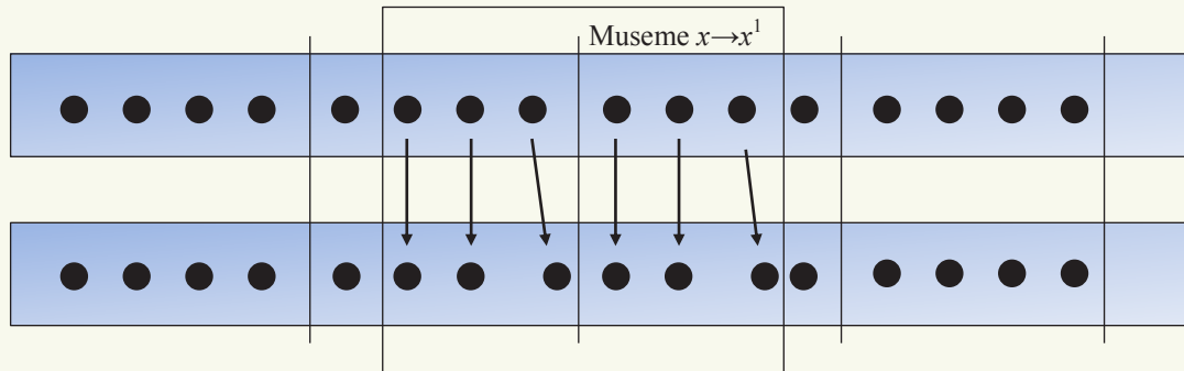
Figure 3. Paraphrase
