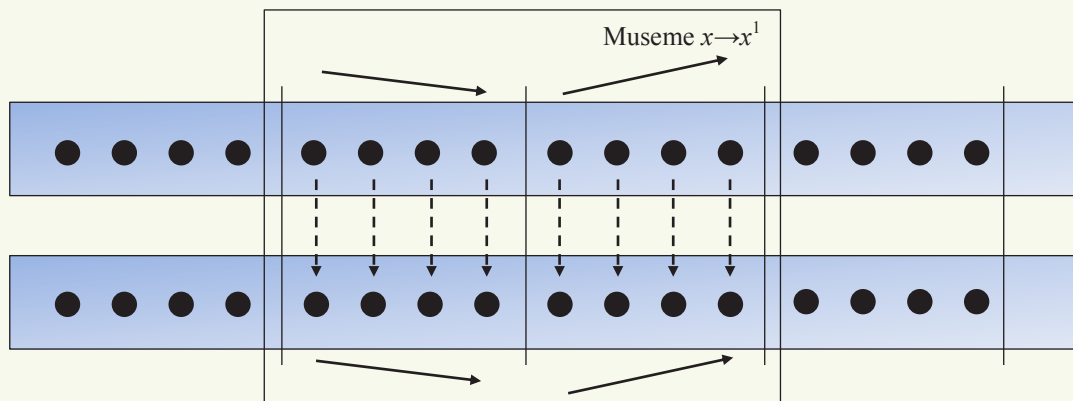
Figure 4. Likeness
