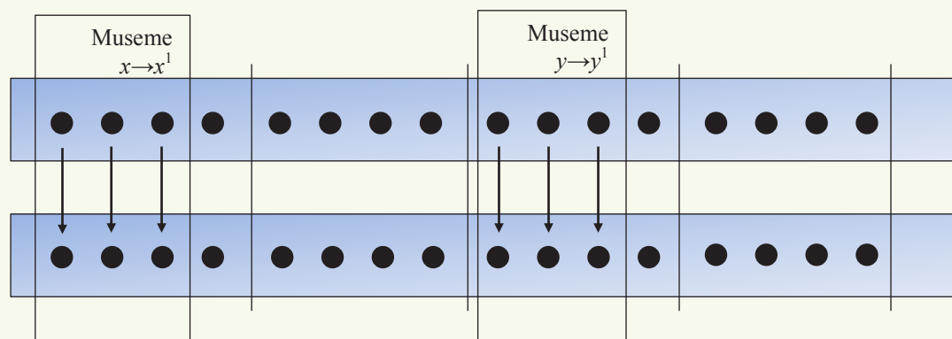
Figure 6. Commonality
