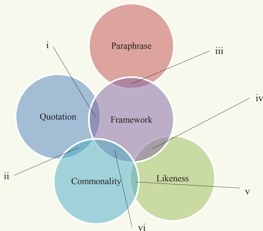
Figure 7. Categorical intersection
