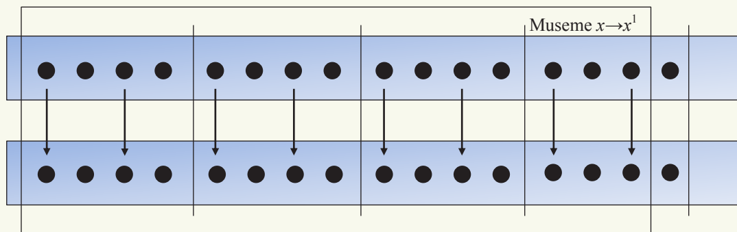
Figure 5. Framework
